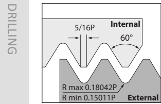
UNJ Internal
