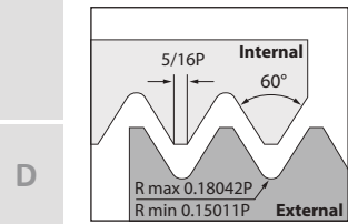
UNJ External
