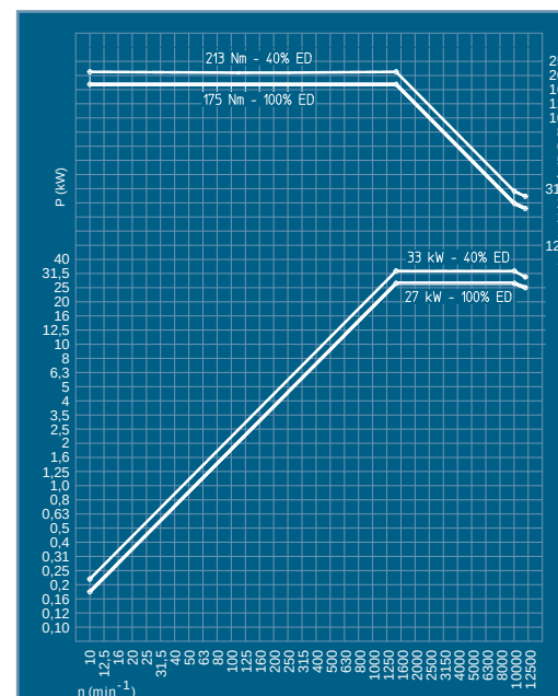
Milling spindle 33(27) kW - 12000 min⁻¹
