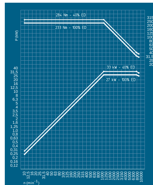
Milling spindle 33(27) kW - 9000 min⁻¹
