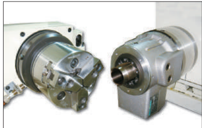
Hydraulic 3-Jaw Chuck + Rotary Cylinder
