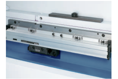
Heidenhain Sub- \mu\text{m} Linear Scale for X-axis (Standard)
