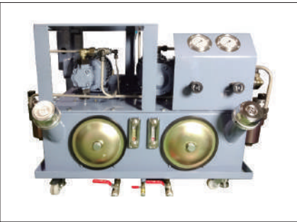
Hydraulic Tank with Pump
