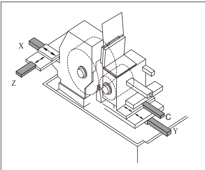
4 AXES X : Grinding wheel auto dressing (vertical) Z : Grinding wheel auto dressing (horizontal) C : Regulating wheel upper slide auto infeed Y : Regulating wheel lower slide auto infeed and compensation.
