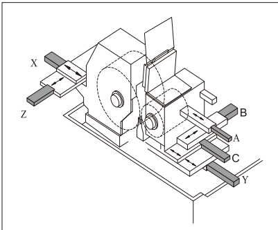
6 AXES X : Grinding wheel auto dressing (vertical) Z : Grinding wheel auto dressing (horizontal) A : Regulating wheel auto dressing (vertical) B :Regulating wheel auto. dressing (horizontal) C : Regulating wheel upper slide auto infeed Y : Regulating wheel lower slide auto infeed and compensation.
