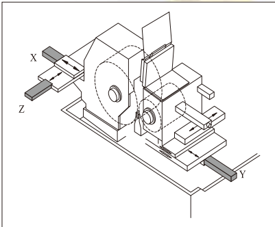
3 AXES X: Grinding wheel auto dressing (vertical) Z: Grinding wheel auto dressing (horizontal) Y: Regulating wheel lower slide auto infeed and compensation.
