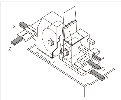
5 AXES X : Grinding wheel auto dressing (vertical) Z : Grinding wheel auto dressing (horizontal) A : Regulating wheel auto dressing (horizontal) C : Regulating wheel upper slide auto infeed Y : Regulating wheel lower slide auto infeed and compensation.
