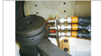
Workpiece chucked indicator device
