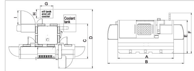
GU-32CNC Series
