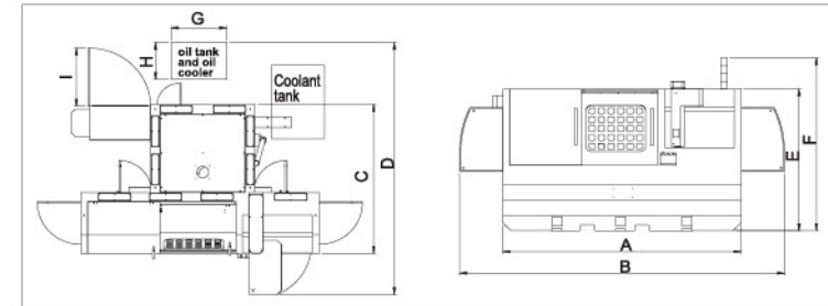
GUH-35CNC Series
