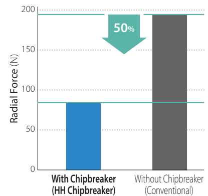
Cutting Force Comparison (Internal Evaluation)
