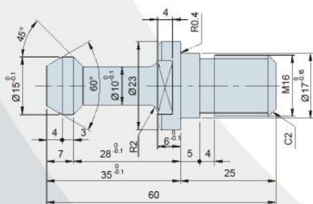
BT-40
