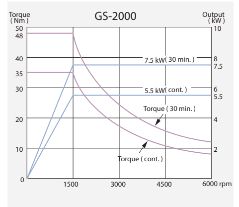
Sub-spindle Output
