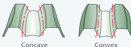
Curvic Coupling
