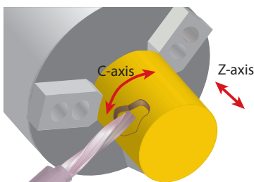
Cylindrical Interpolation.
